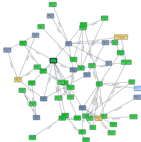
Complex, interconnected system: dependency graph of a bug
